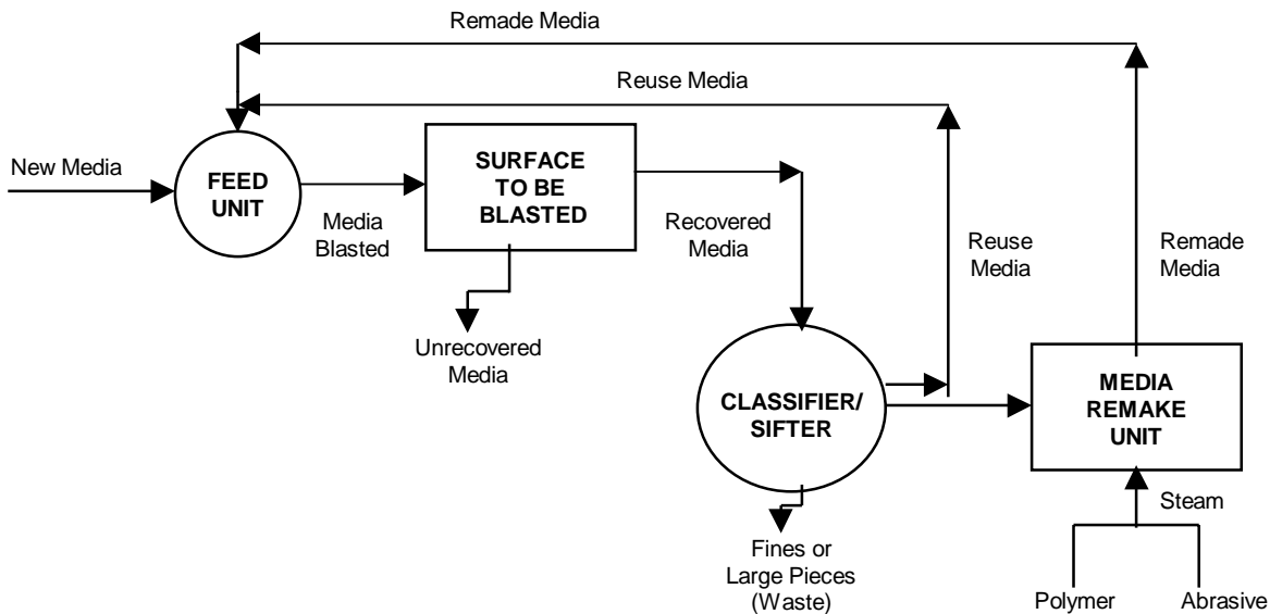
Figure 3. Process Flow Chart for ARMS
